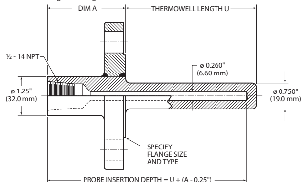
TW1219 Flanged Straight Thermowell
