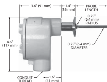
PROBE ASSEMBLY
