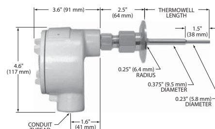
THERMOWELL ASSEMBLY
